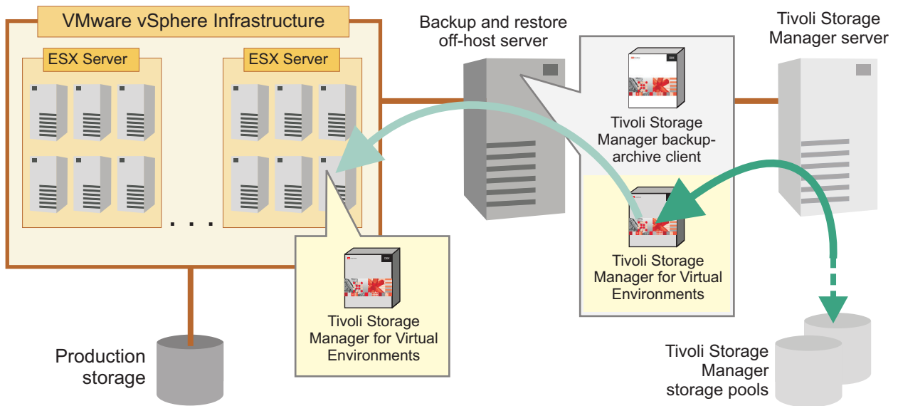
Figure 10. In-guest file-level restore for Linux
