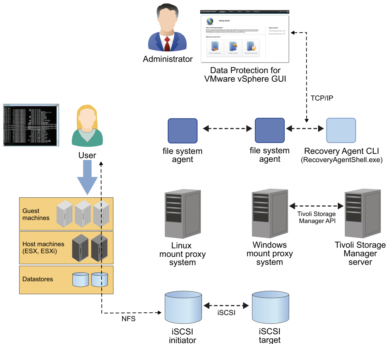
Figure 6. Tivoli Storage Manager for Virtual Environments file-level restore operation for a Linux virtual machine.
