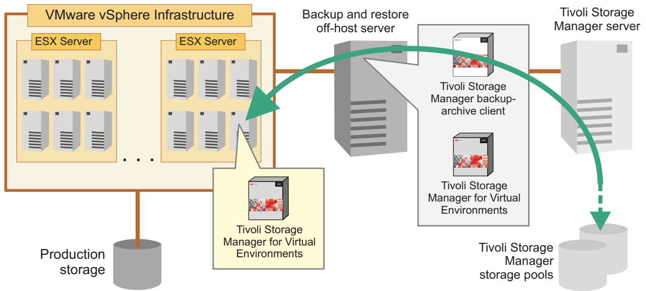
Figure 11. In-guest instant restore for Windows
