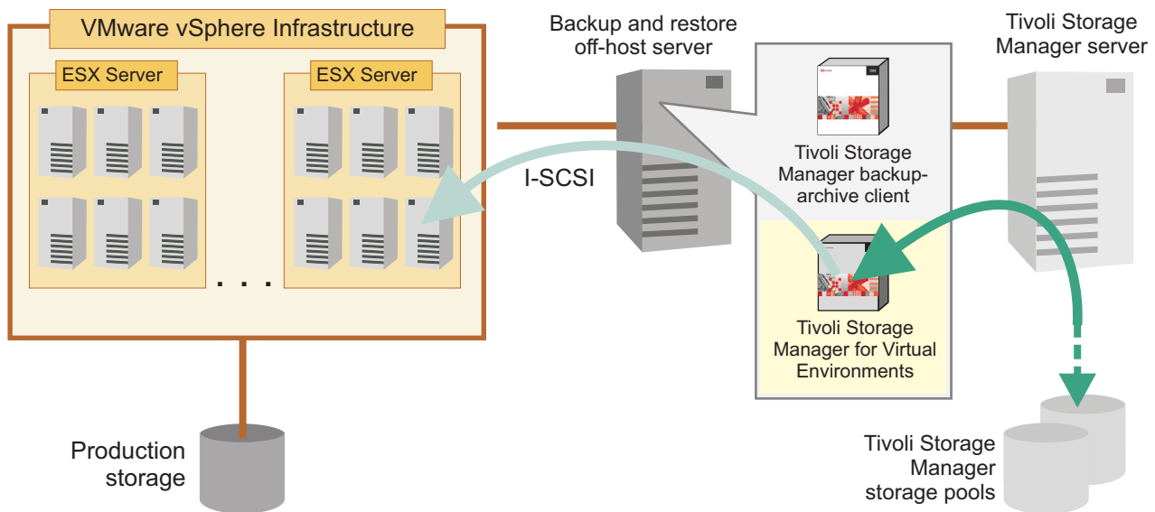
Figure 13. Off-host iSCSI target
