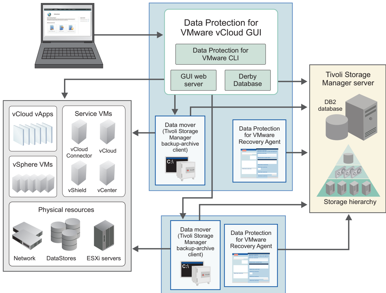
Figure 2. Tivoli Storage Manager for Virtual Environments system components in a VMware vCloud Director user environment
